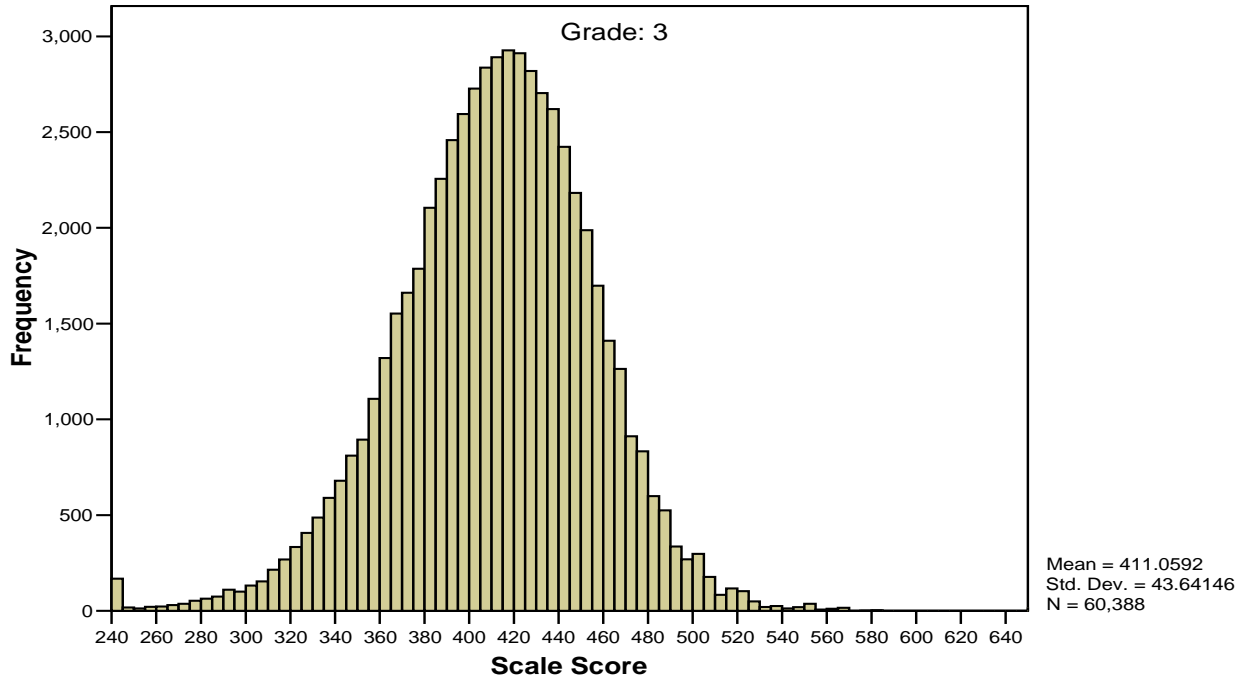
Figure G1 Scale Score Distribution for Grade 3 Mathematics
