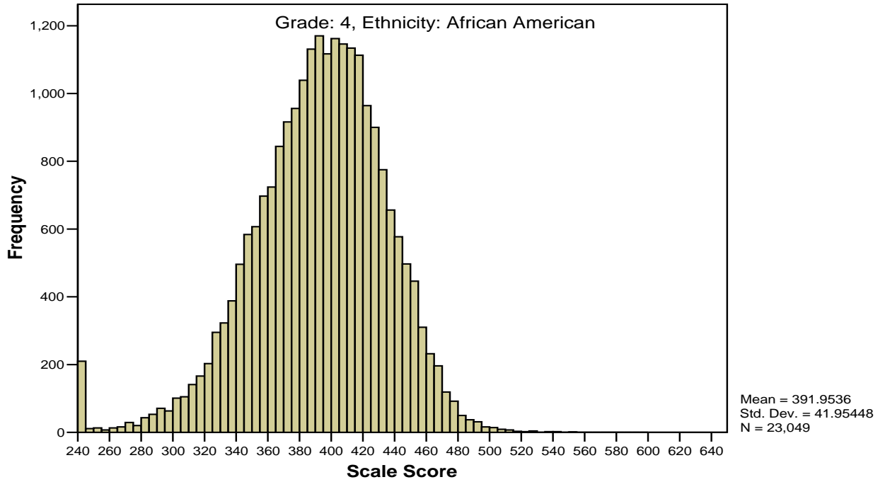
Figure G6 Scale Score Distribution for Grade 4 Mathematics by Ethnicity
