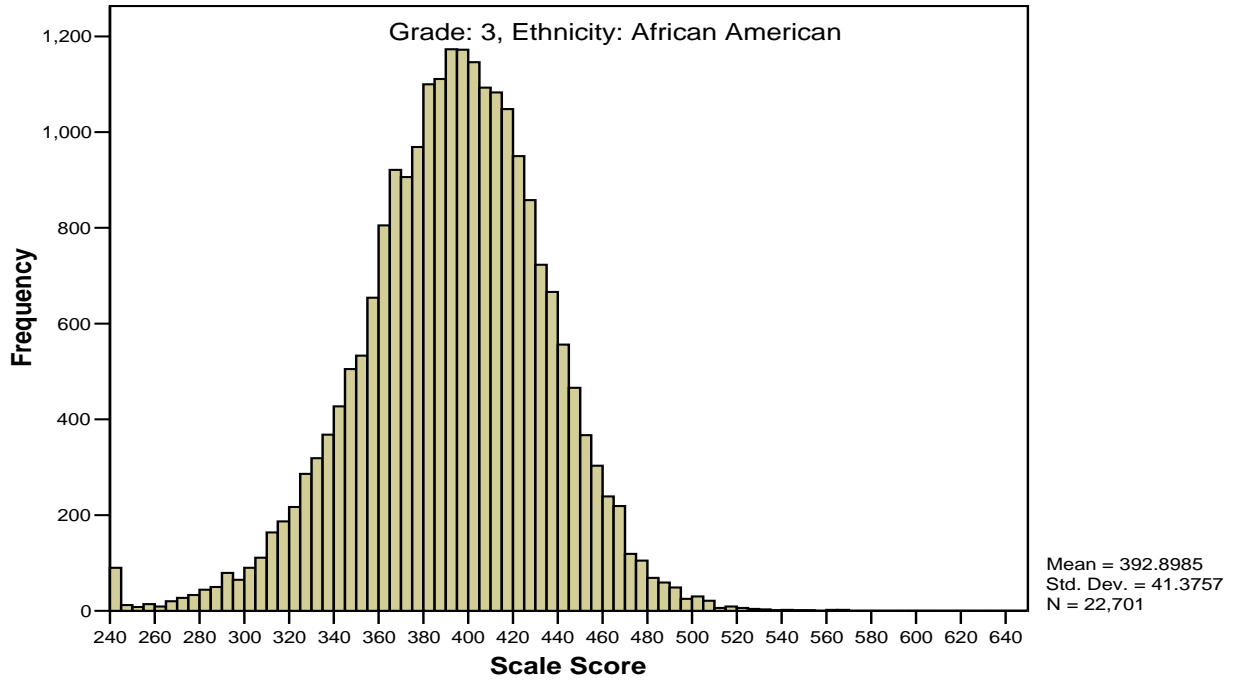
Figure G3 Scale Score Distribution for Grade 3 Mathematics by Ethnicity
