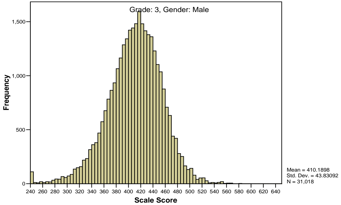
Figure G2 Scale Score Distribution for Grade 3 Mathematics by Gender
