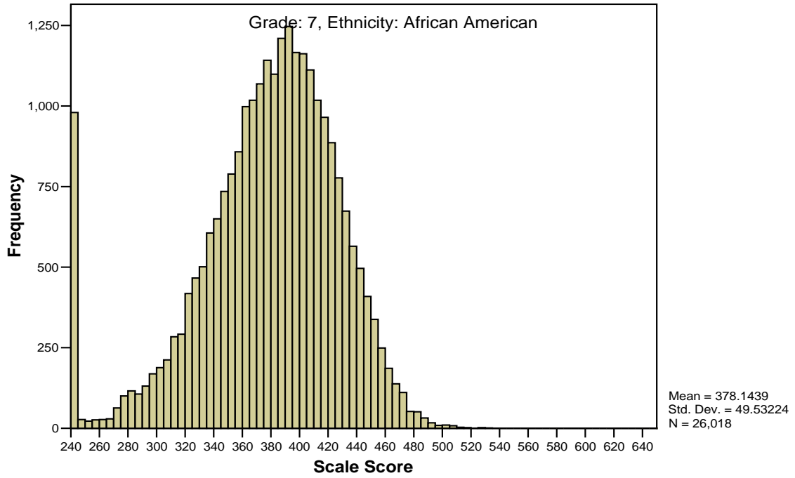
Figure G15 Scale Score Distribution for Grade 7 Mathematics by Ethnicity
