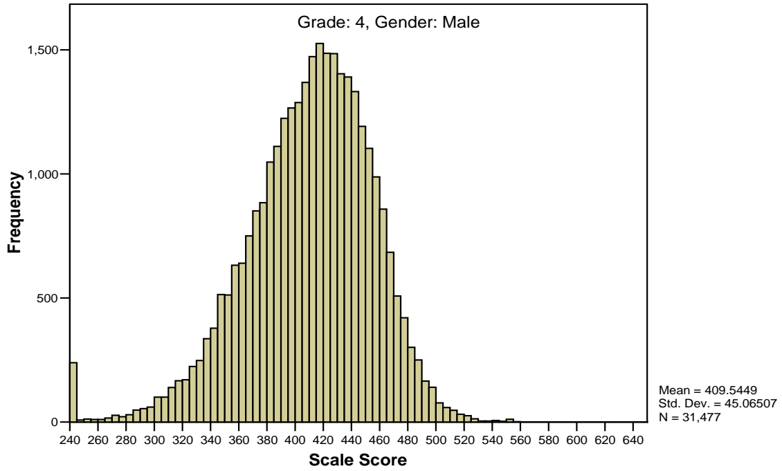
Figure G5 Scale Score Distribution for Grade 4 Mathematics by Gender
