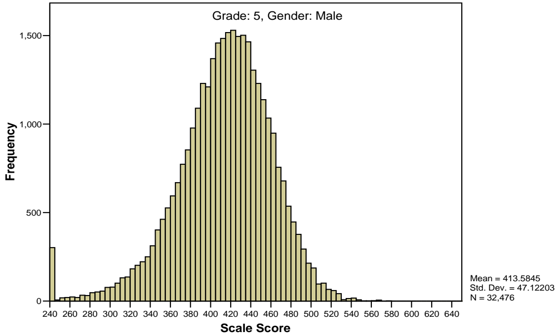
Figure G8 Scale Score Distribution for Grade 5 Mathematics by Gender
