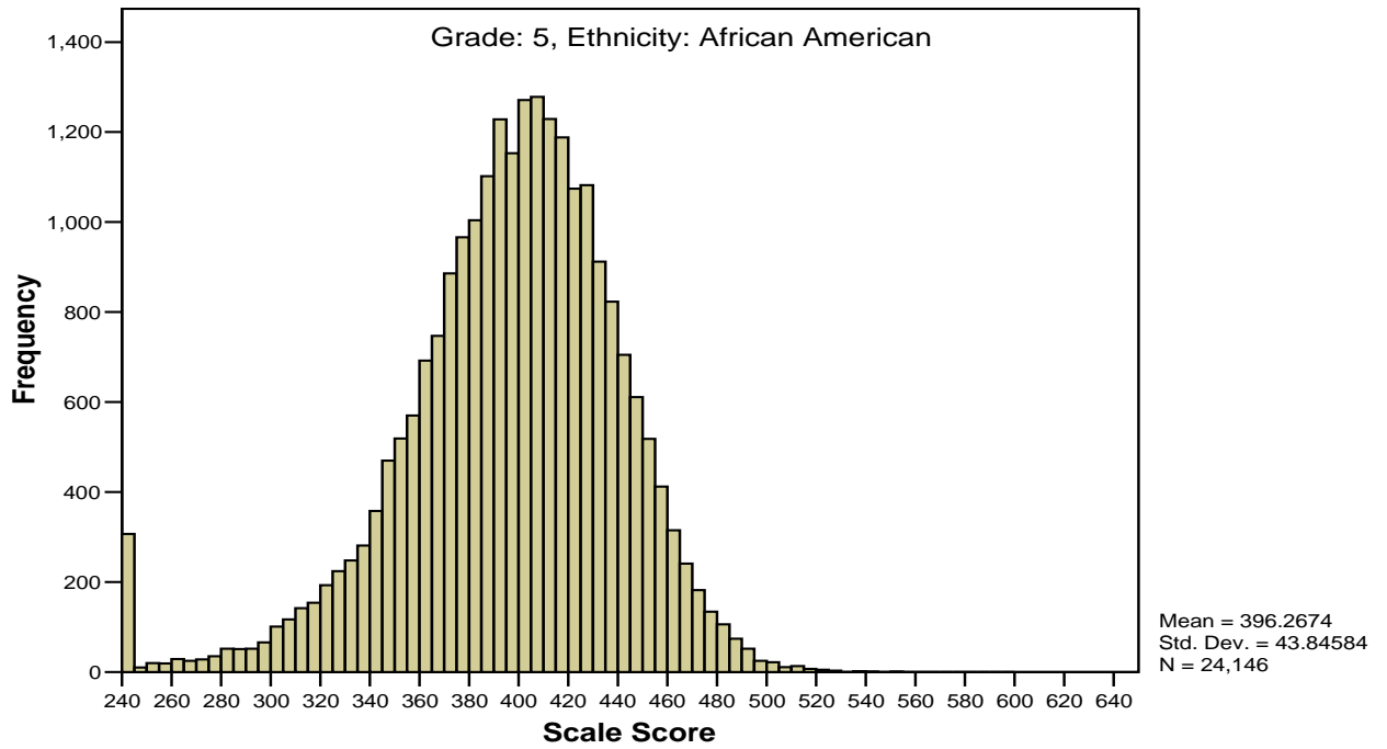
Figure G9 Scale Score Distribution for Grade 5 Mathematics by Ethnicity
