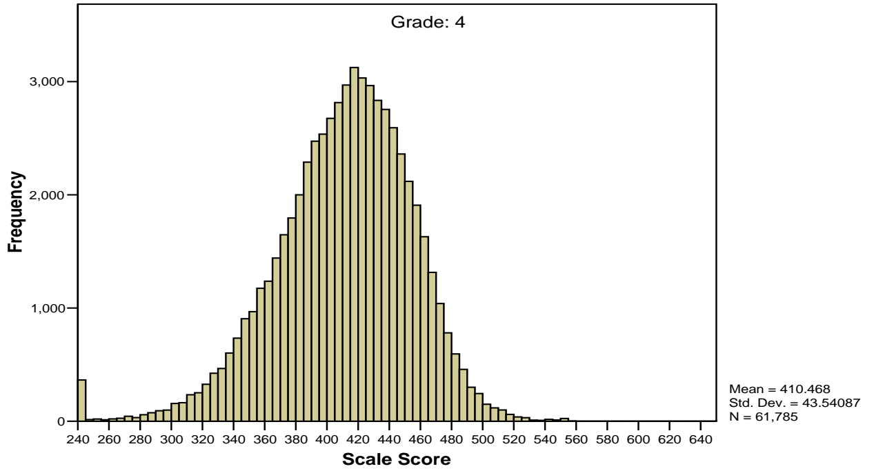
Figure G4 Scale Score Distribution for Grade 4 Mathematics
