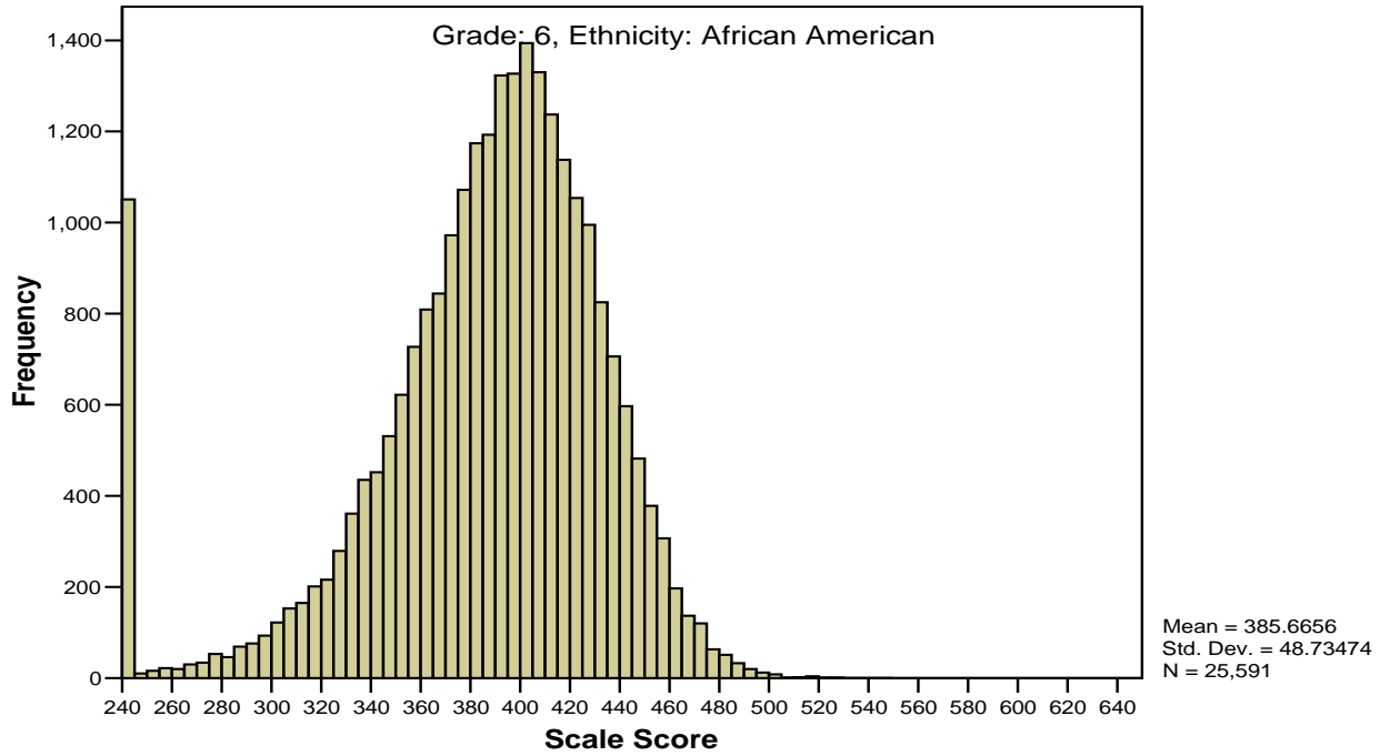
Figure G12 Scale Score Distribution for Grade 6 Mathematics by Ethnicity
