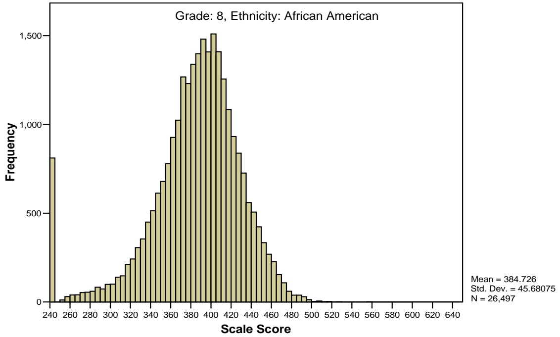
Figure G18 Scale Score Distribution for Grade 8 Mathematics by Ethnicity
