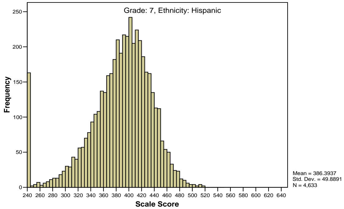
Figure G15 (cont.) Scale Score Distribution for Grade 7 Mathematics by Ethnicity
