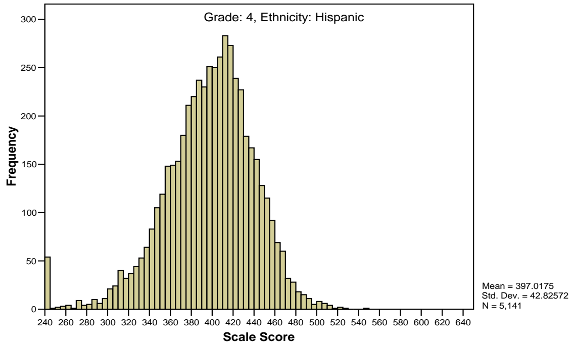
Figure G6 (cont.) Scale Score Distribution for Grade 4 Mathematics by Ethnicity
