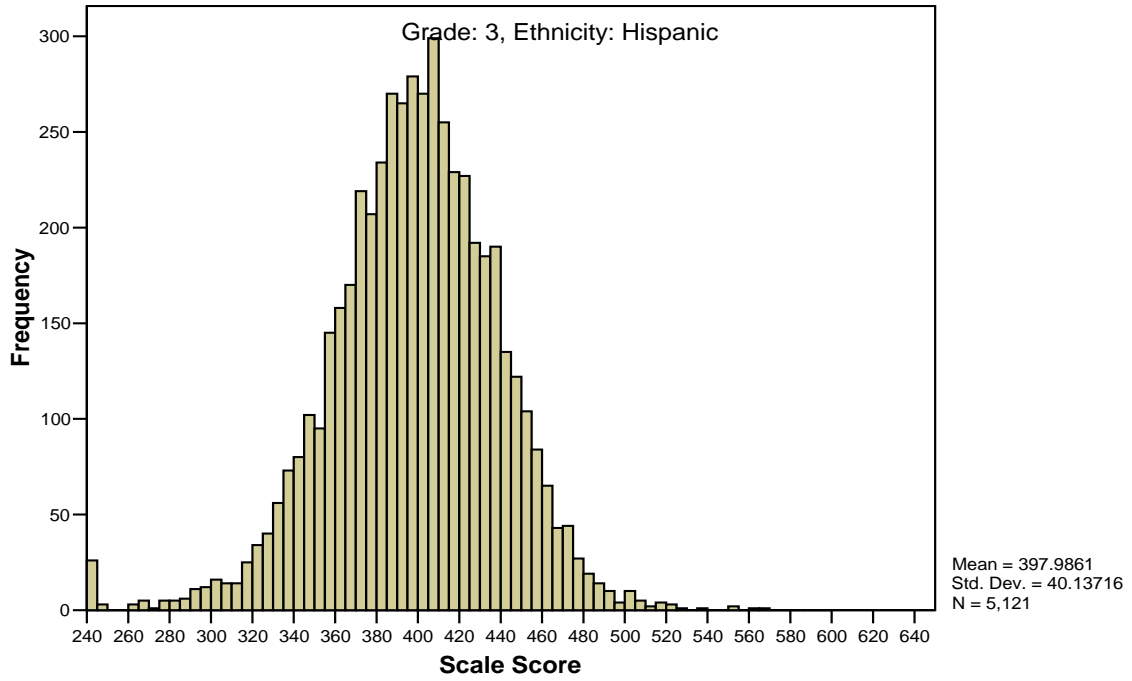
Figure G3 (cont.) Scale Score Distribution for Grade 3 Mathematics by Ethnicity
