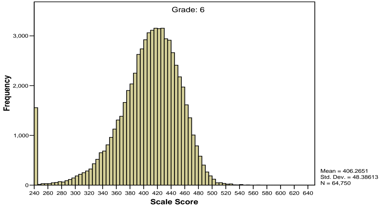
Figure G10 Scale Score Distribution for Grade 6 Mathematics
