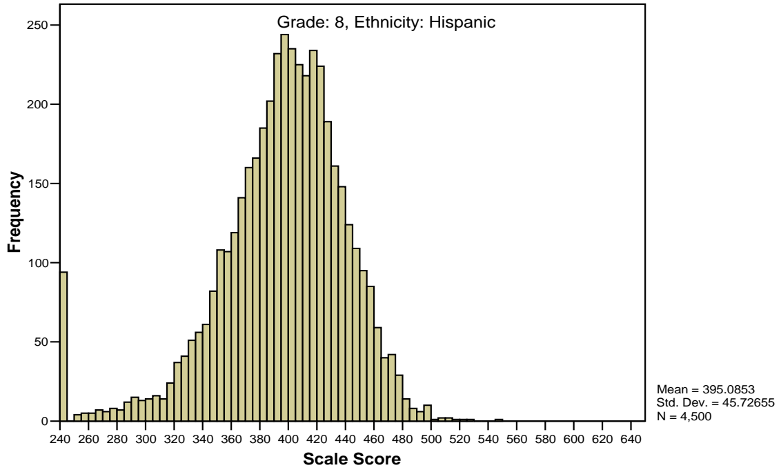
Figure G18 (cont.) Scale Score Distribution for Grade 8 Mathematics by Ethnicity
