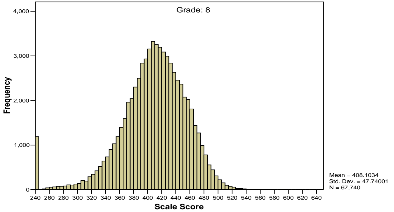
Figure G16 Scale Score Distribution for Grade 8 Mathematics
