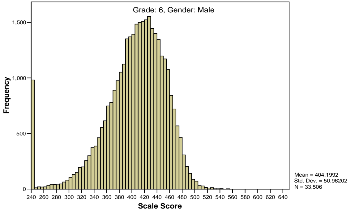
Figure G11 Scale Score Distribution for Grade 6 Mathematics by Gender
