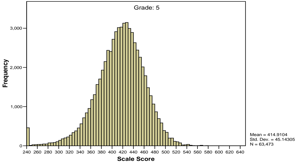
Figure G7 Scale Score Distribution for Grade 5 Mathematics
