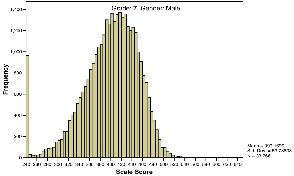
Figure G14 Scale Score Distribution for Grade 7 Mathematics by Gender
