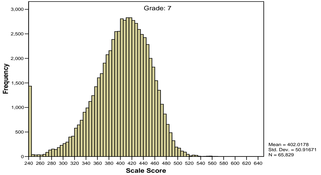
Figure G13 Scale Score Distribution for Grade 7 Mathematics
