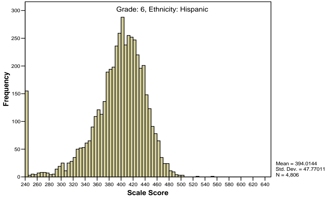
Figure G12 (cont.) Scale Score Distribution for Grade 6 Mathematics by Ethnicity
