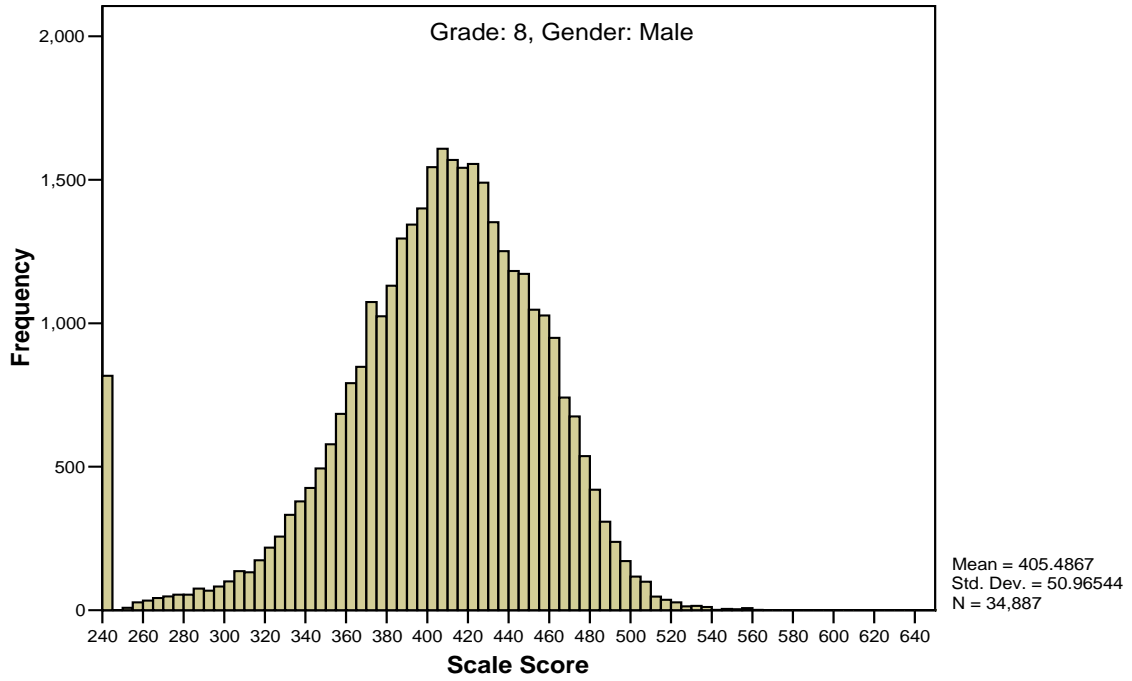
Figure G17 Scale Score Distribution for Grade 8 Mathematics by Gender
