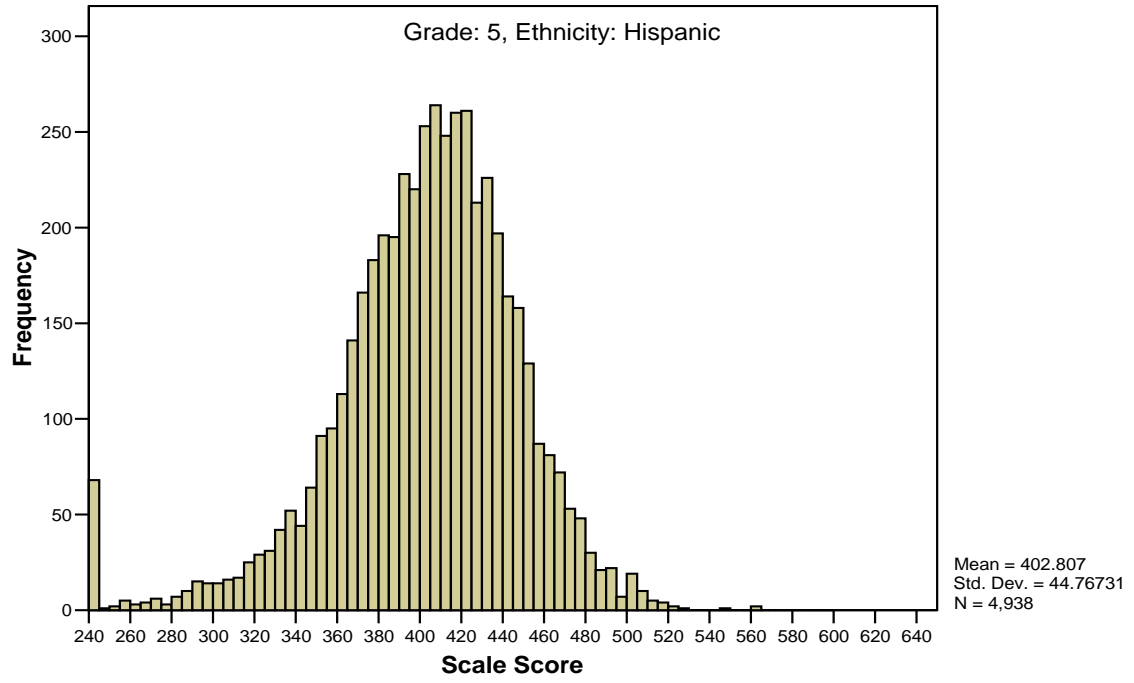
Figure G9 (cont.) Scale Score Distribution for Grade 5 Mathematics by Ethnicity
