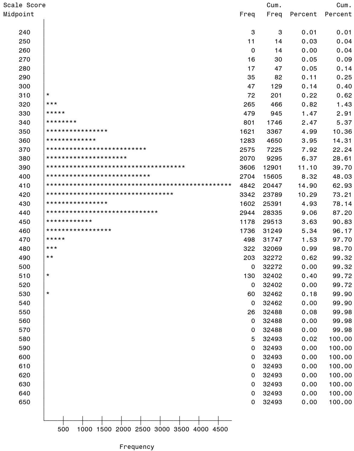
Figure B.33 Year 2006 Scale Score Distribution: Grade 7 Form A
